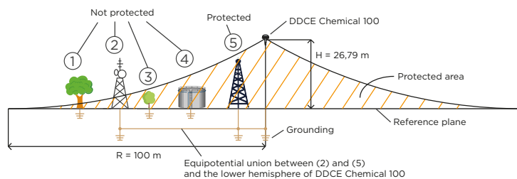
Figure 2. Example area protected by a DDCE. Profile view.
