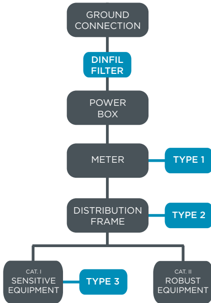
Figure 3. Electrical installation diagram.
