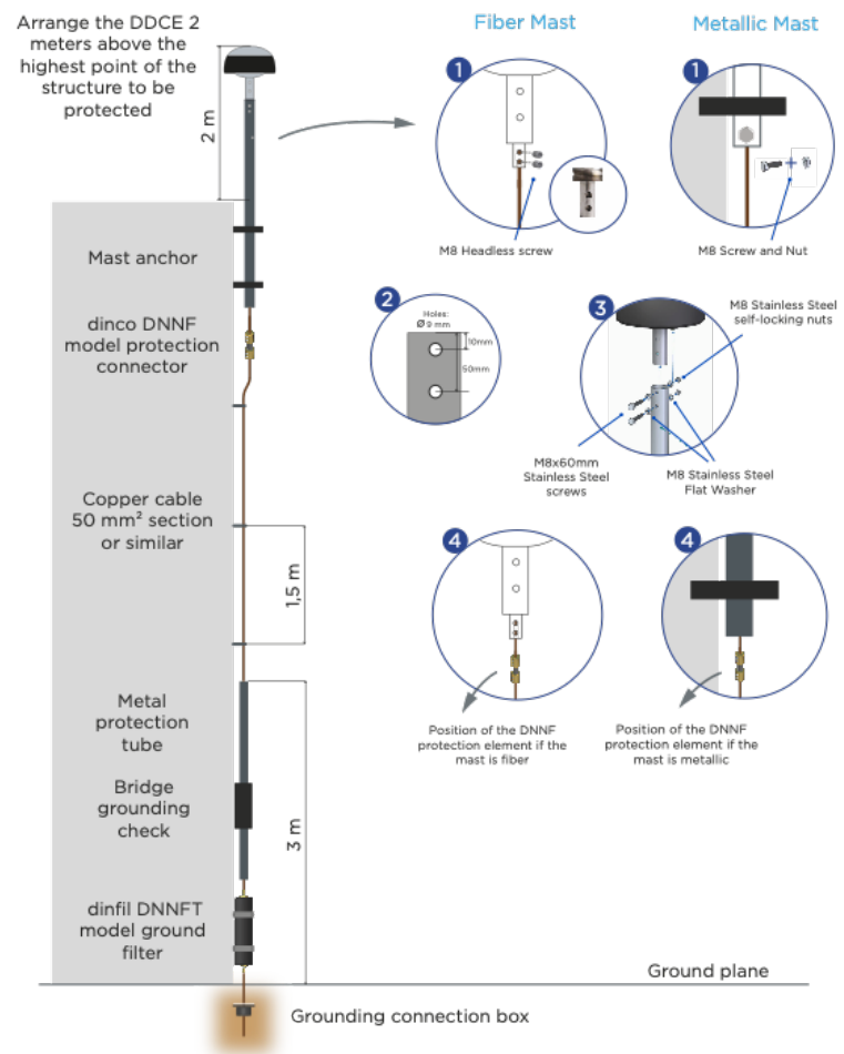
Figure 4. Installation of the DDCE Chemical 100.
